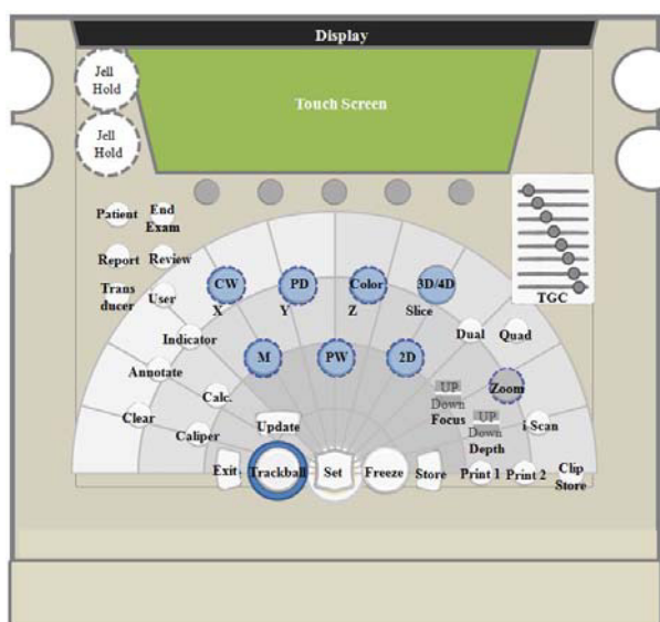
Figure 7. One alternative control panel layout. Based on anthropometric control design guideline [2], minimal distance between buttons was kept at 10mm while the size of specific control types were guided as the following: Trackball (50mm), Push buttons (20mm), Rotary push buttons (24mm), Set/Exit/Update buttons (20mm).
